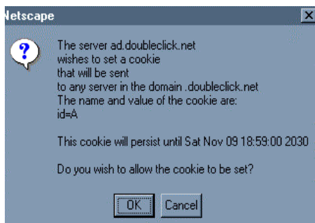
Figure 1: NS 3.04 Cookie Warning Dialog Box
